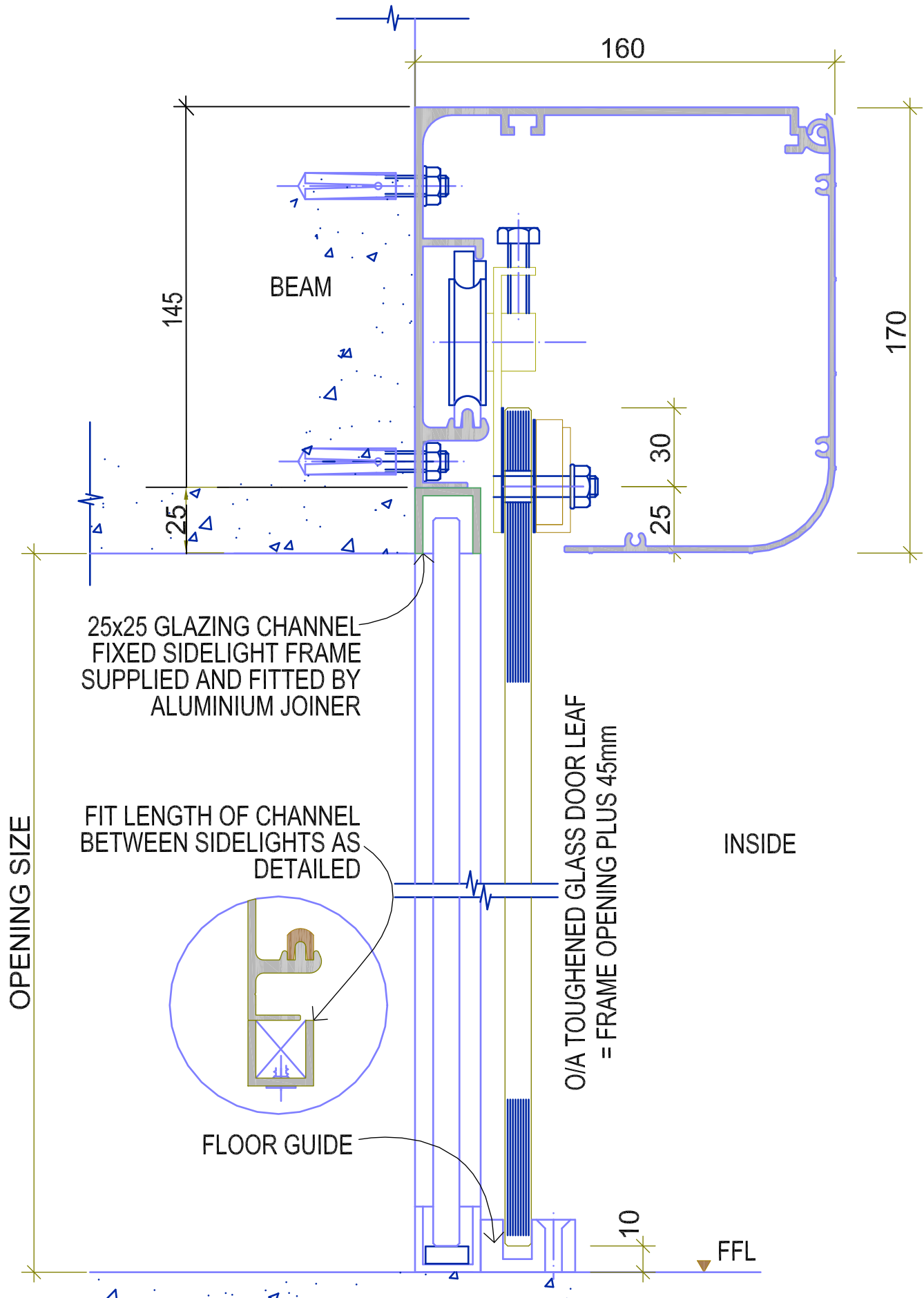
HALF FULL SIZE VERTICAL SECTION THROUGH ULTRASLIDE SD AUTOMATIC DOOR OPERATOR. BEAM MOUNTED WITH 'FRAMELESS' GLASS DOORS AND SIDELIGHTS
